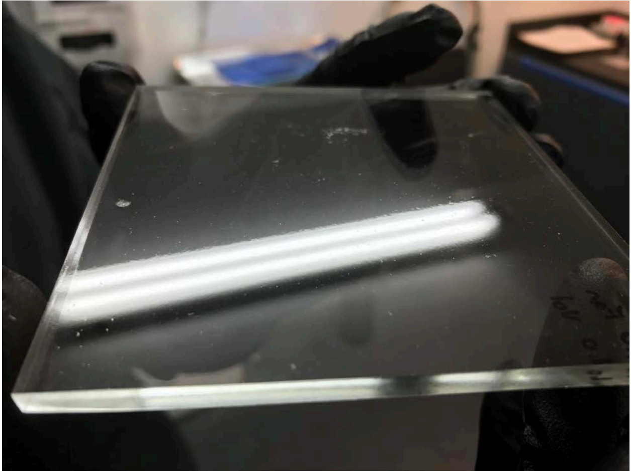
Example of “orange peel” on glass. This is the rippled effect seen around the reflection of the overhead light.
