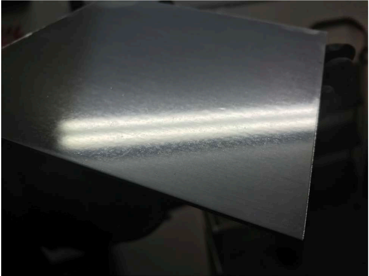
Example of “orange peel” on aluminum.
